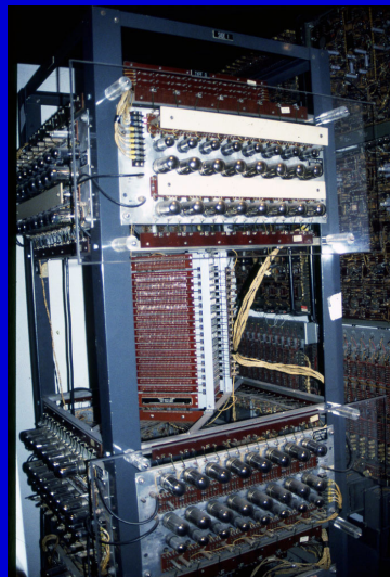
Bottom - Vacuum tube storage / Core memory stack / Core memory plane
