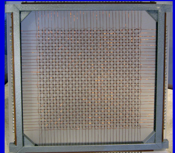
Bottom - Vacuum tube storage / Core memory stack / Core memory plane
